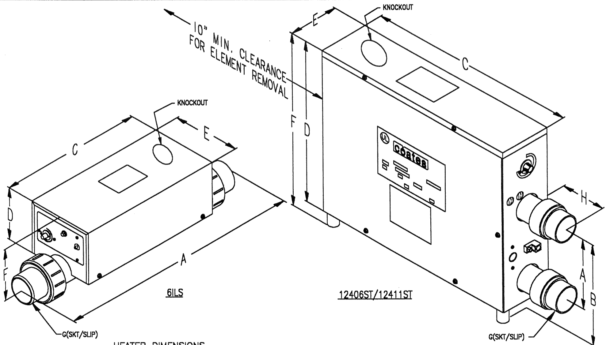
HEATER DIMENSIONS
